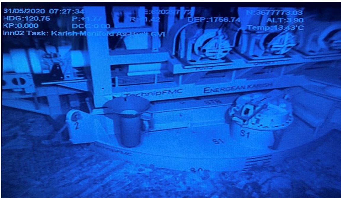
Karish Manifold
